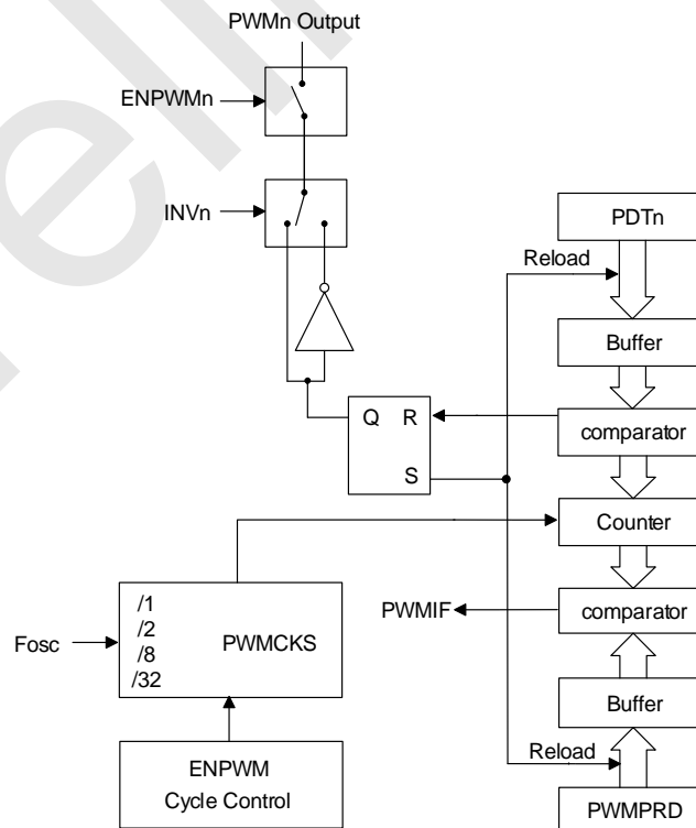
The SC92F84AX PWM Independent Mode Block Diagram
