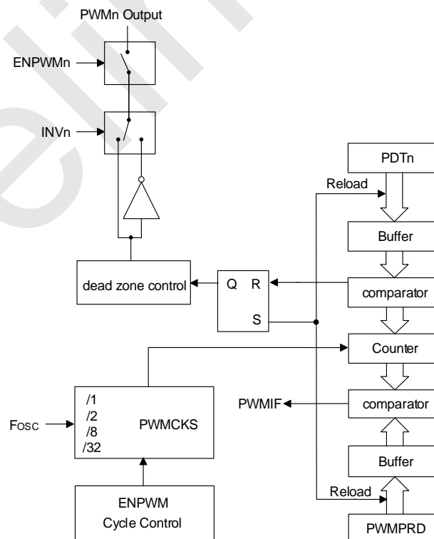
The SC92F84AX PWM block Diagram
