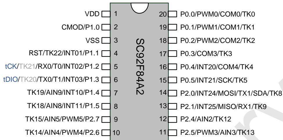
The SC92F84A2 Pin Diagram
