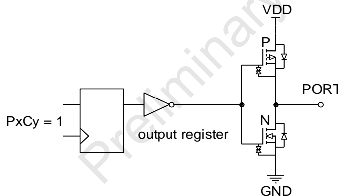
Strong Push-pull Output Mode
