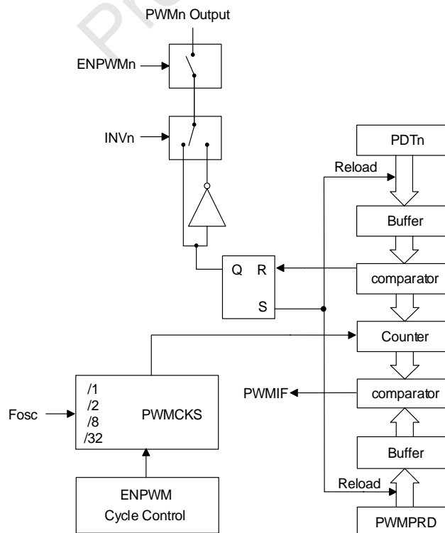
The SC92F846XB PWM Independent Mode Block Diagram
