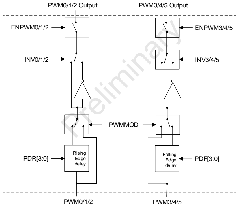
The SC92F846XB PWM Complementary Mode Block Diagram
