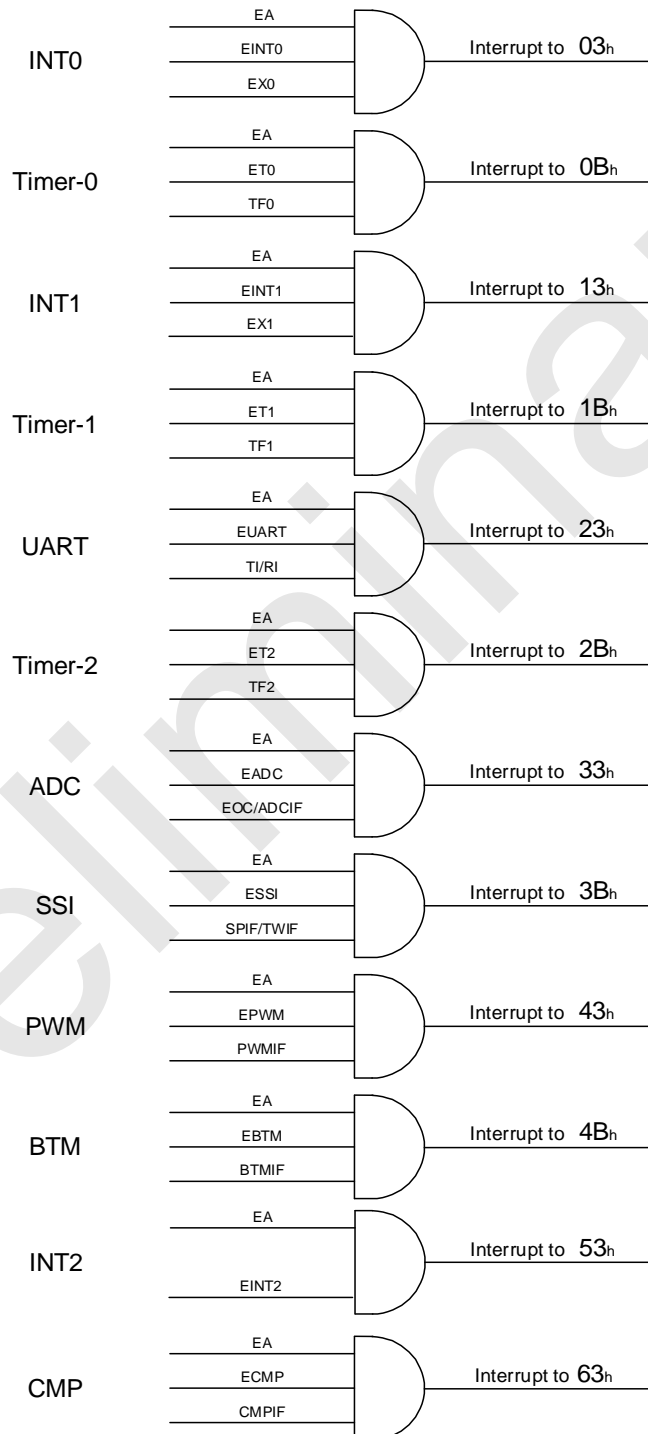
SC92F759X Interrupt structure and vector
