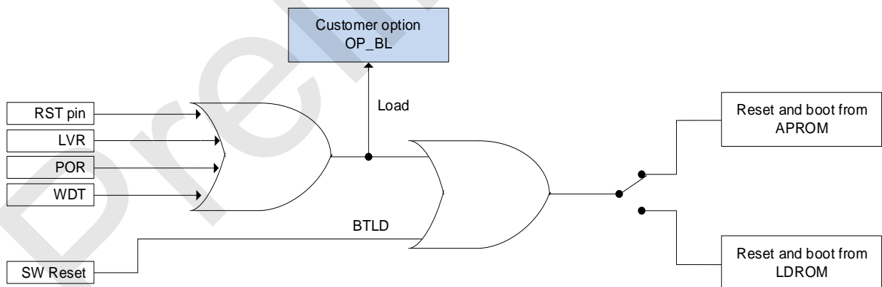
SC92F759X's boot area switch after reset
