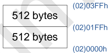
SC92F759X EEPROM Sector Partition diagram
