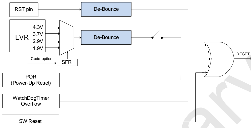
SC92F759X Reset circuit diagram
