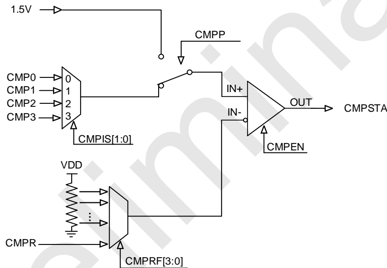
Block Diagram of Analog Comparator
