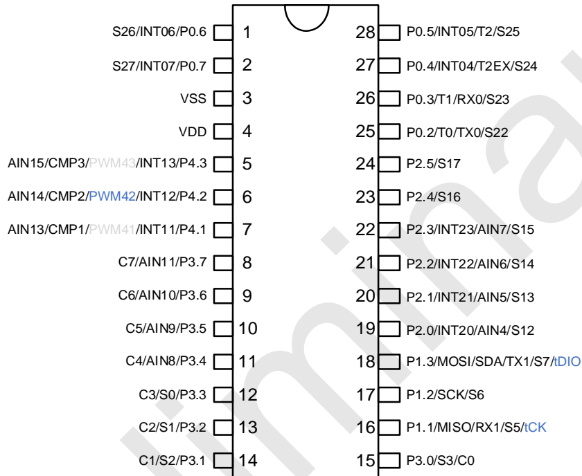
28 Pin Diagram
