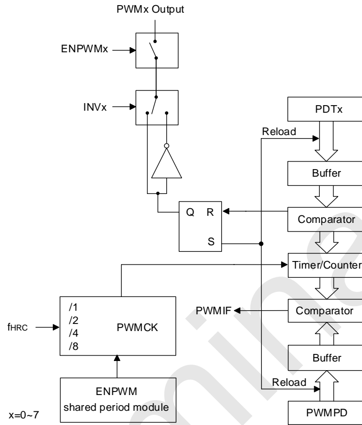
SC92F759X PWM Structure Diagram
