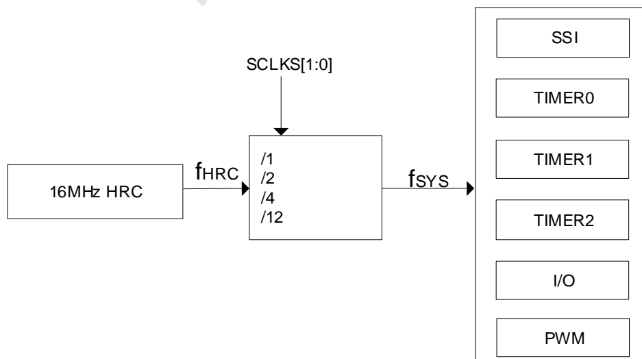
The SC92F742X Internal Clock Relationship
