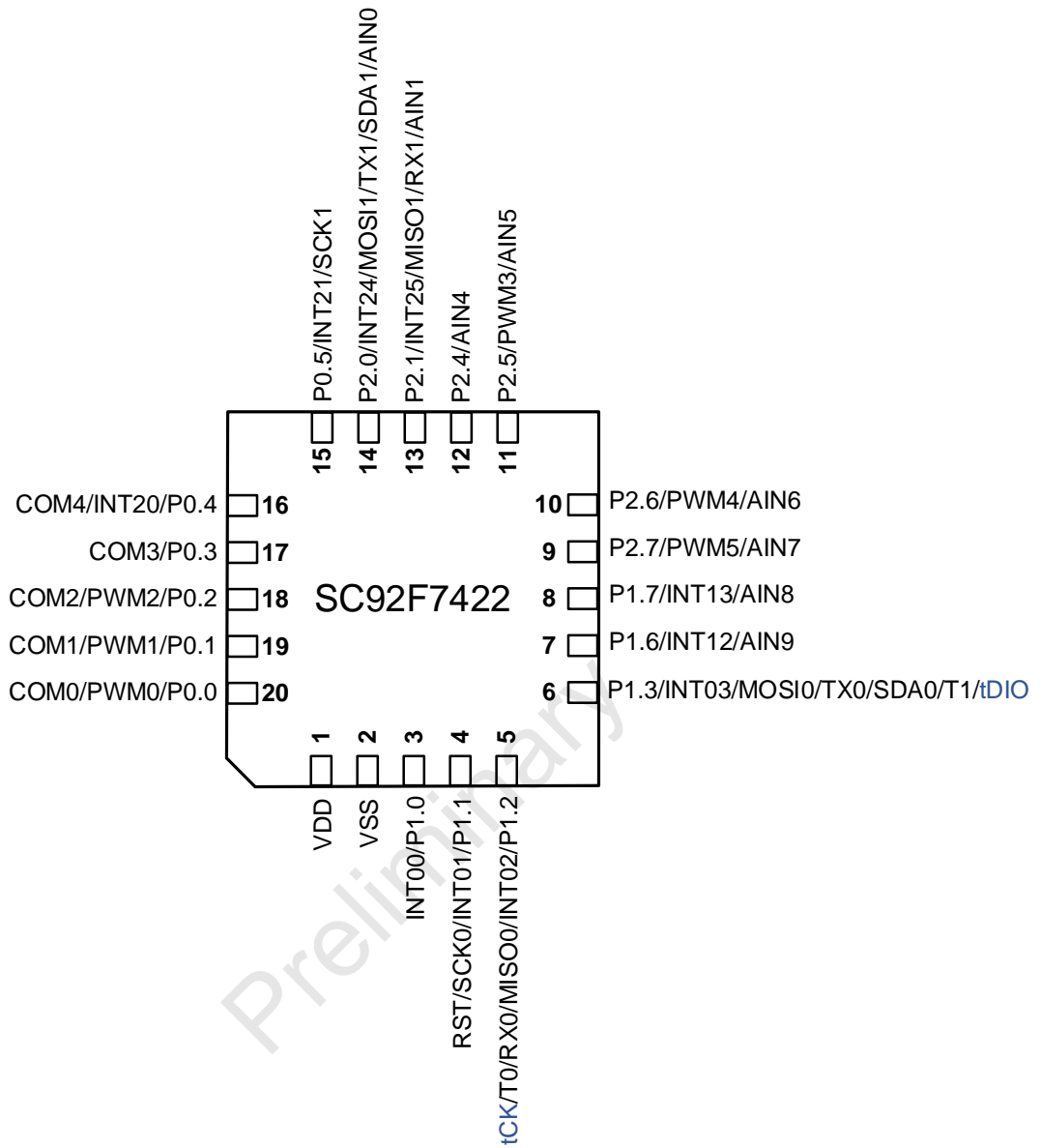
The SC92F7422 Pin Diagram (QFN20)
